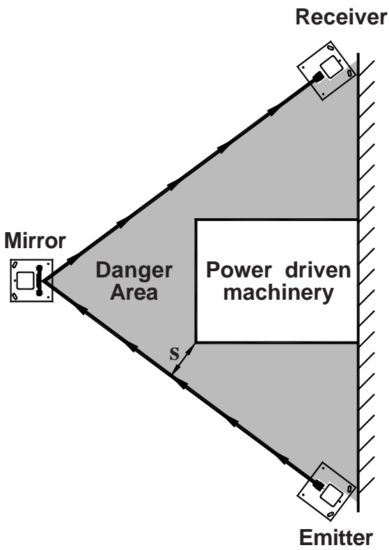
Figure 18 - Incorrect use of two sided guarding
