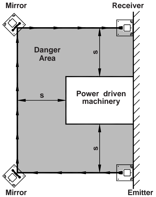
Figure 17 - Guarding a three sided area
