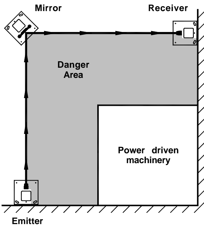
Figure 9 - 'L' shaped protection (when the curtain protects two sides with the addition of one mirror unit).
