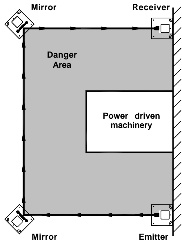
Figure 10 - 'U' shaped protection (when the curtain protects three sides with the addition of two mirror units).
