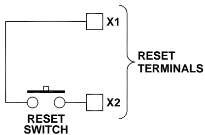
Figure 7 - Manual Reset
