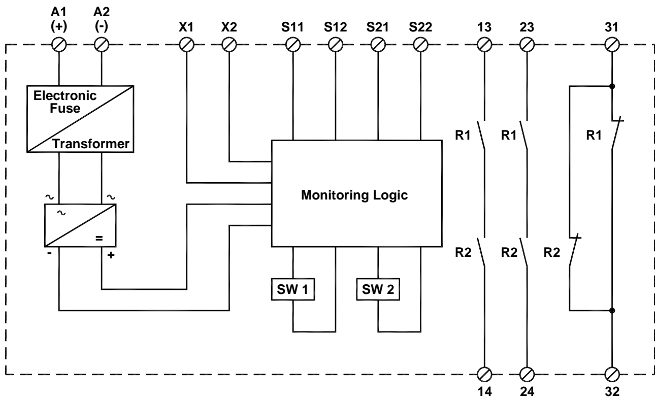
Figure 3 - PSSR/2 Schematic
